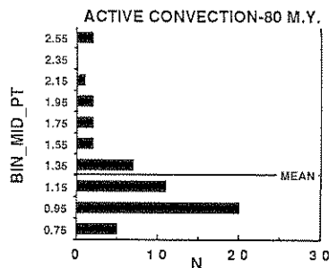
Fig. 4. Heat flow ratio histograms (Right): No convection. X^* is 56.5%. (Left): Convecting, conductively blanketed
