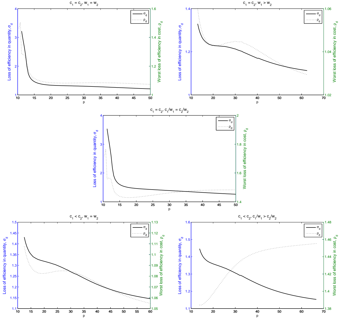
Figure 5: The loss of efficiency in quantity, \sigma_d , and the worst loss of efficiency in cost, \rho_d , are illustrated here for two hospitals ( n = 2 ). Parameters (c_1, c_2, w_1, w_2) are given respectively: (5, 5, 0.5, 0.5) , (5, 5, 0.6, 0.4) , (4, 6, 0.4, 0.6) , (4, 6, 0.5, 0.5) and (4, 6, 0.3, 0.7) .
