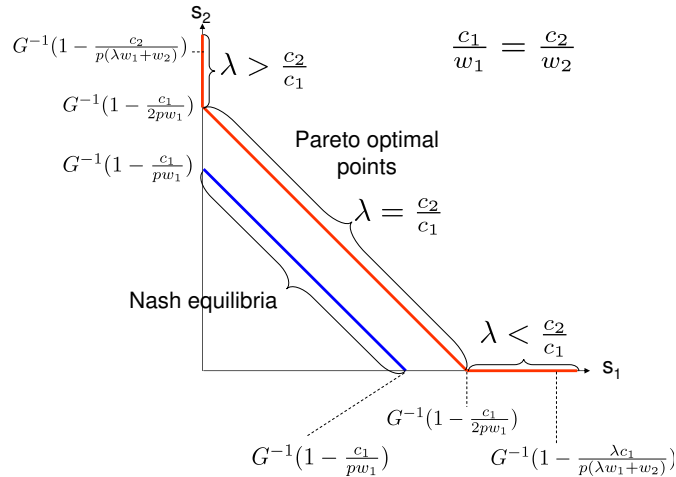
Figure 3: Nash equilibria and Pareto optimal points illustrated in the case with n = 2 .
