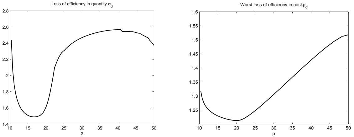
Figure 6: A two-hospital example showing that the ratio of loss of efficiency in cost and quantity is not necessarily monotonically decreasing in the penalty cost p . Parameters used: L = 3 , demand distributions with means = [100 300 500] and standard deviations [30 70 120], c = [4 6] , w = [0.4 0.6] , q = [0.8 0.1 0.1] .
