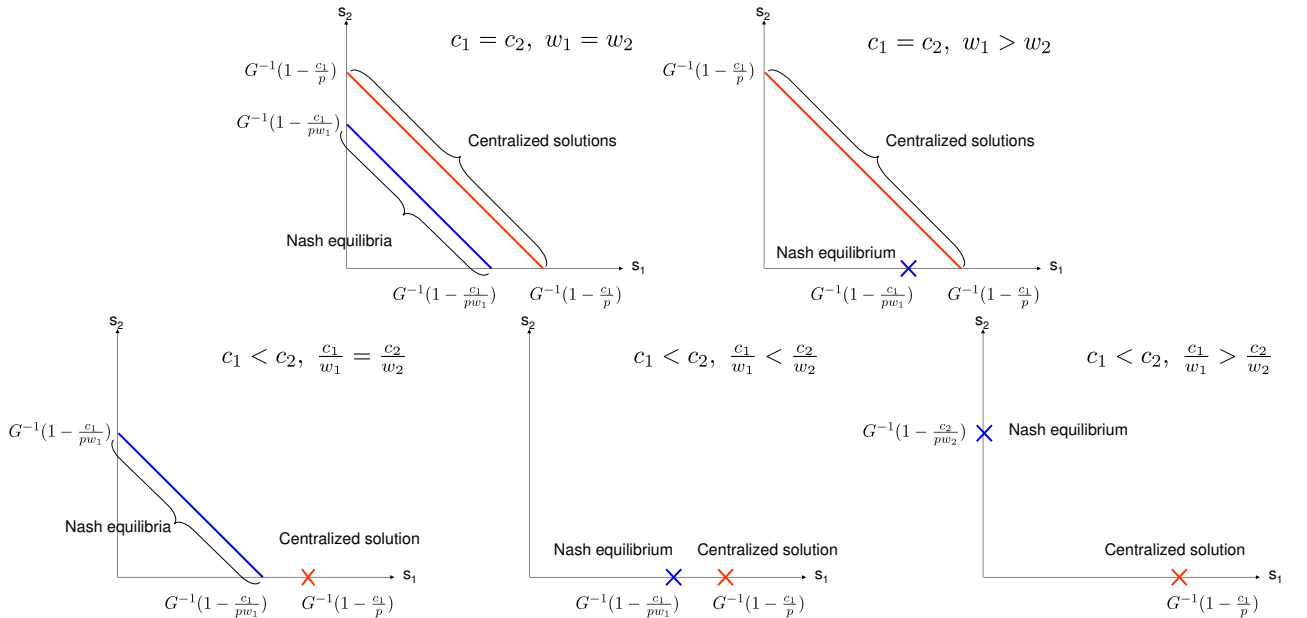
Figure 4: Centralized solution and Nash equilibrium illustrated in the case with n = 2 .
