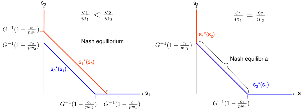
Figure 2: Nash equilibrium illustrated in the case with n = 2 .
