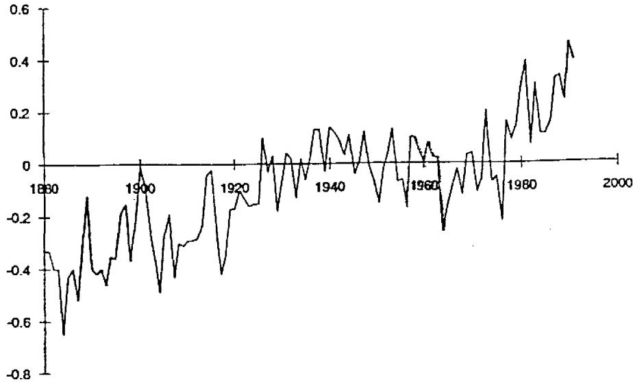
Fig. 1. Temperature 1880–1991.
