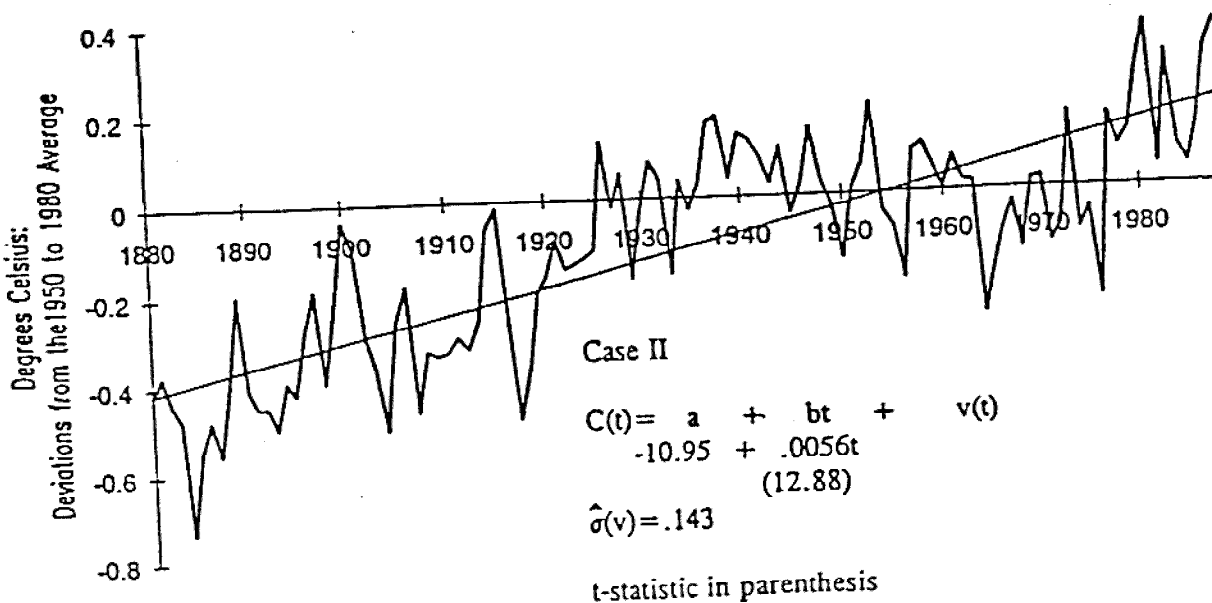
Fig. 2. Annual temperature time series.
