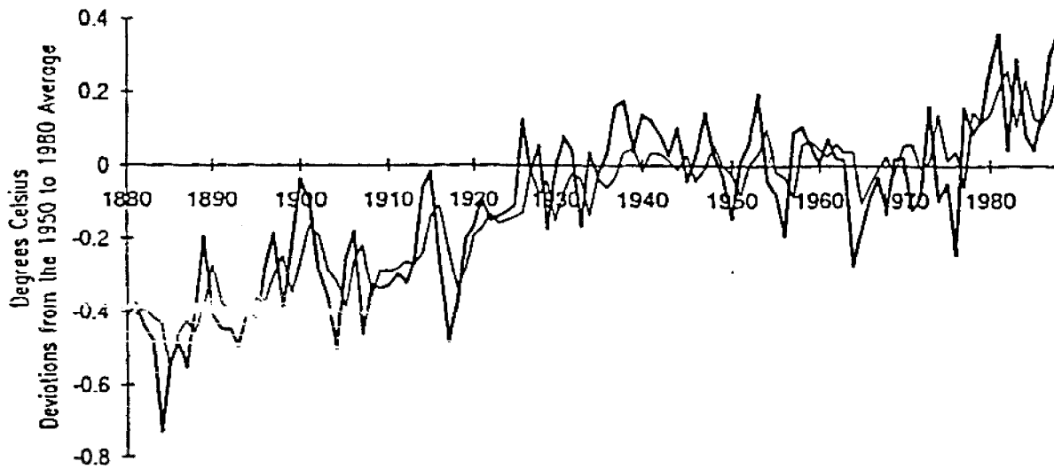
Fig. 4. Fitted and actual temperature Case III.
