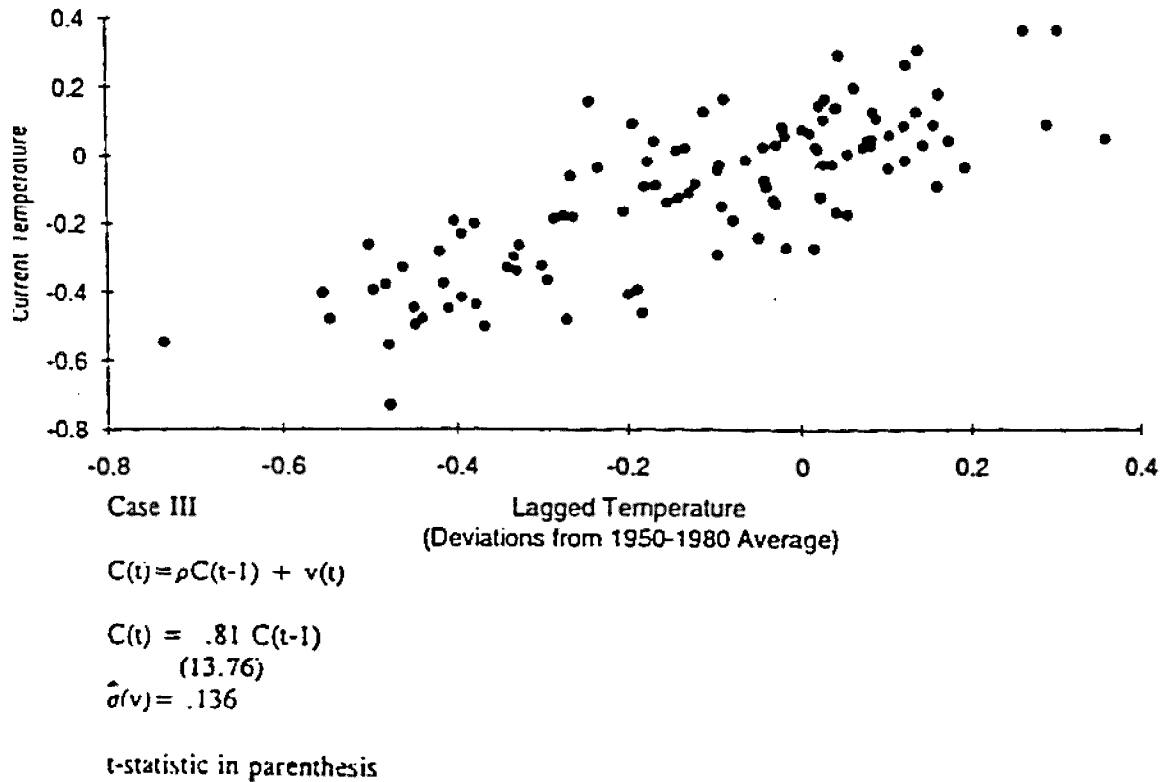
Fig. 3. Current vs lagged temperature.
