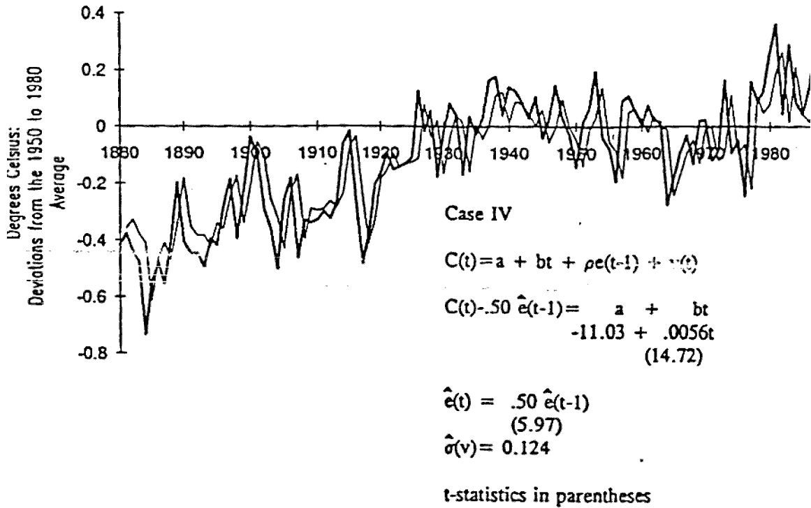
Fig. 6. Fitted and actual temperature Case IV.
