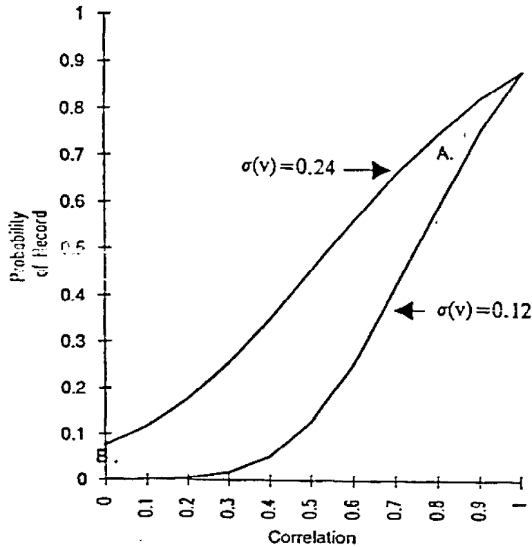
Fig. 5. Record probability as a function of correlation.
