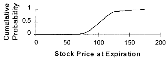
Histogram cdf
