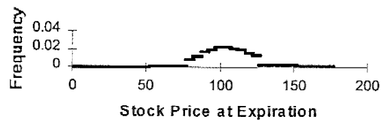
Figure2 Histogram Probability
