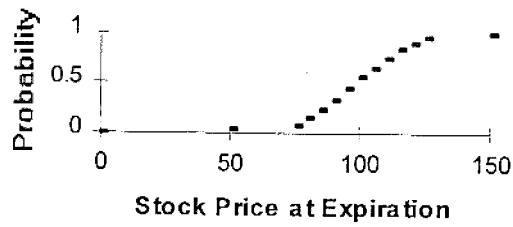
Discrete cdf
