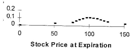
Figure 1 Discrete Probability
